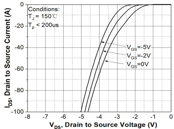
Figure 10. Body Diode Characteristic at T_J = 150^\circ C
